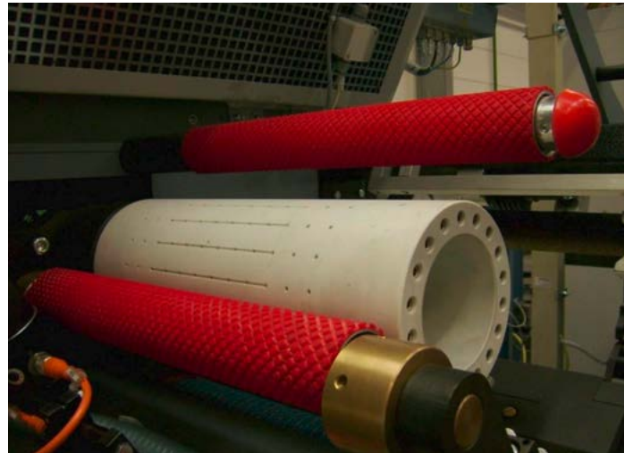
Guide roller in the peel and seal unit
