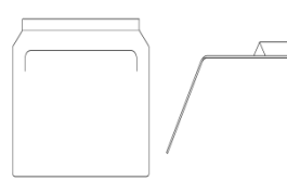
Clamping bar 80°
